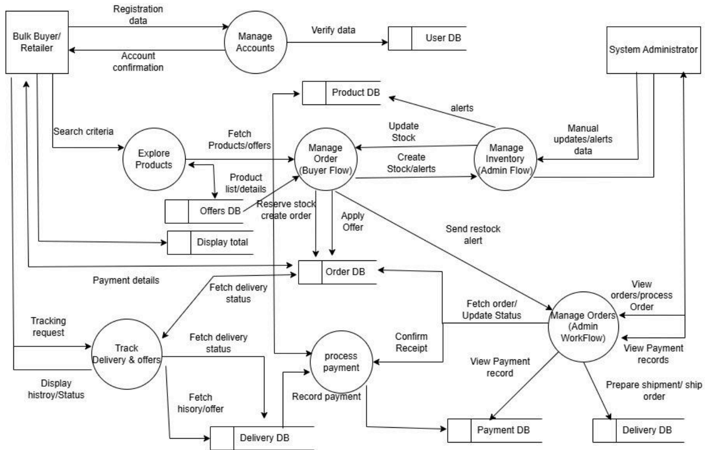
Figure: Data Flow Diagram Level 1
